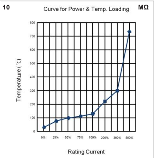
Curve of temp. rise and rated current
